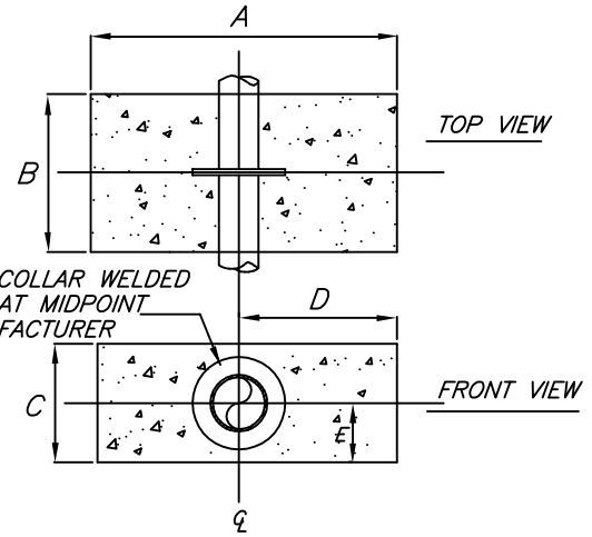
DETAIL "A" DIP ONLY
