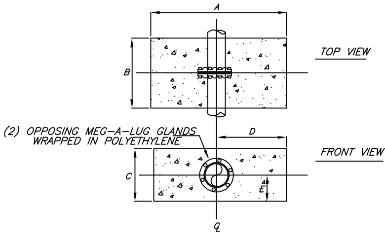
DETAIL "B" DIP ONLY
