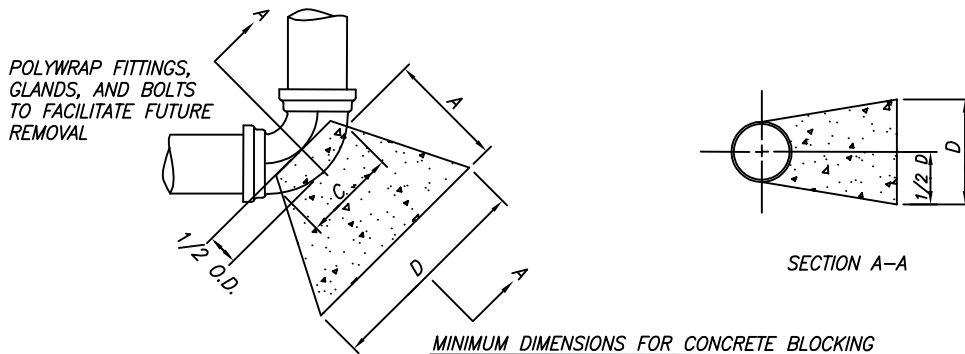
MINIMUM DIMENSIONS FOR CONCRETE BLOCKING
